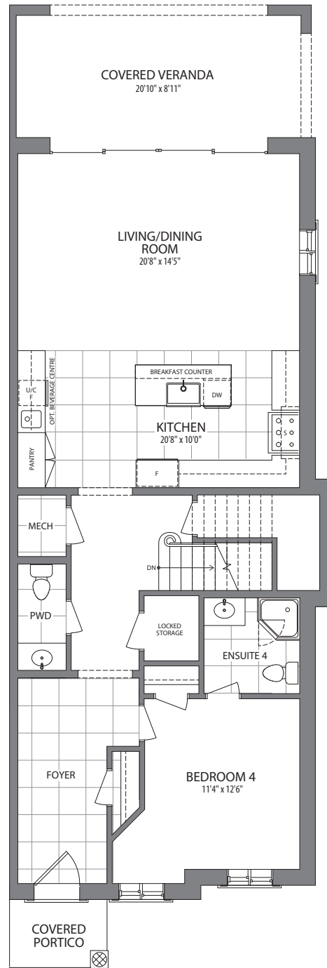
MAIN FLOOR
